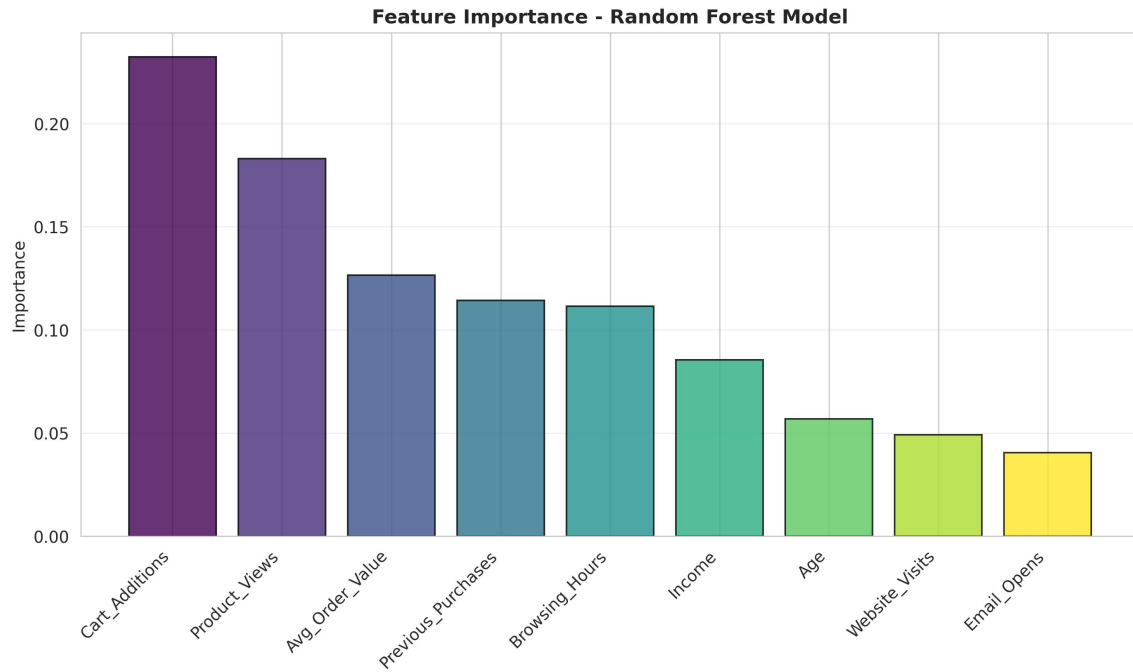
Figure 3: Feature Importance Analysis (Random Forest)
