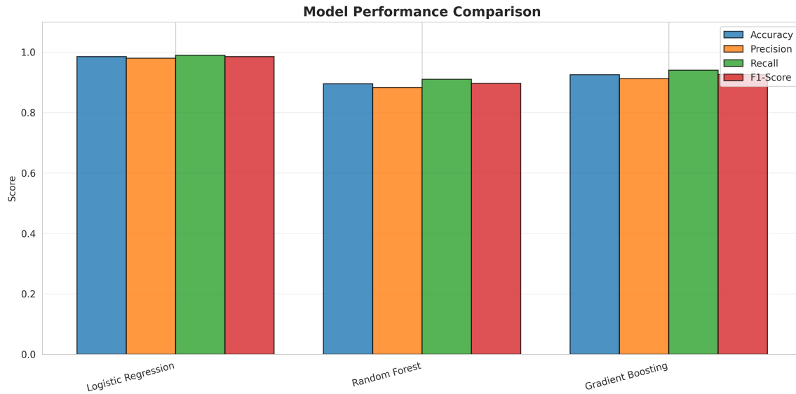
Figure 4: Model Performance Metrics Comparison
