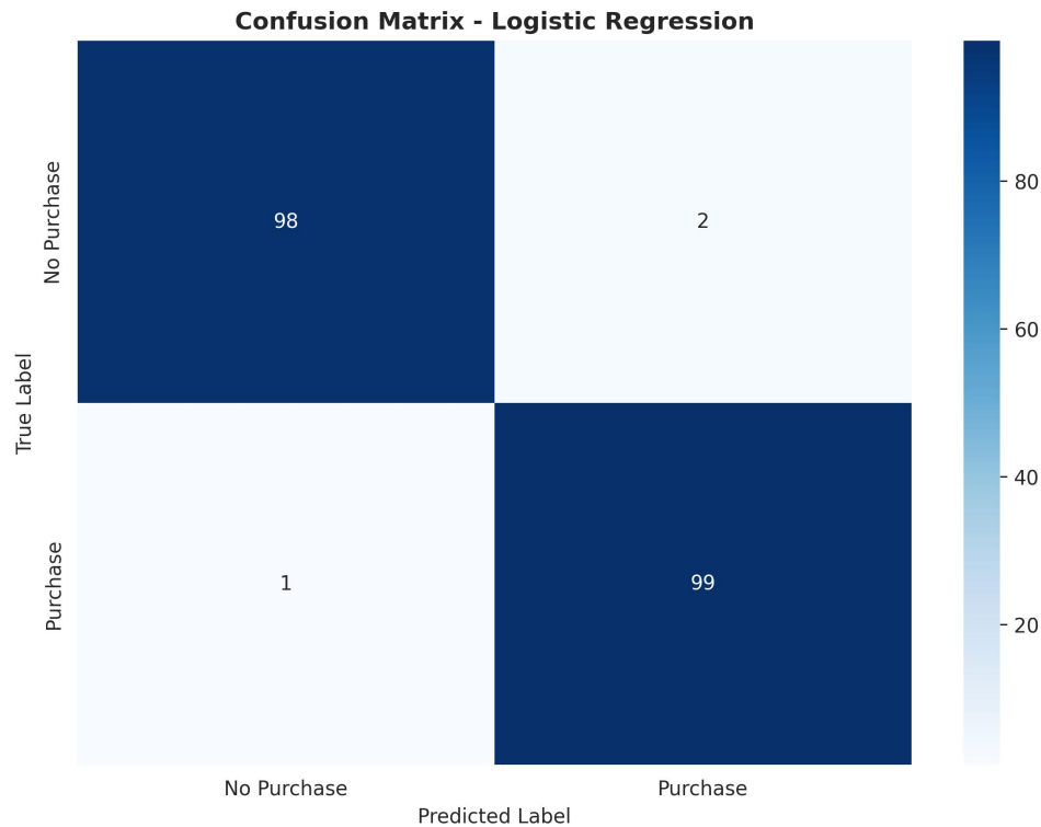
Figure 6: Confusion Matrix for Best Model (Logistic Regression)
